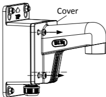
Figure 2-15 Unscrew the Cover
