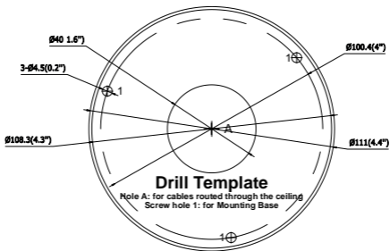
Figure 2-3 Drill Template
