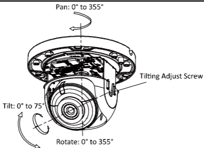
Figure 2-8 Angle Adjustment of Type III and Type VI Camera
