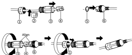
Figure 2-26 Install Waterproof Jacket
