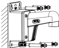
Figure 2-14 Fix the Bracket
