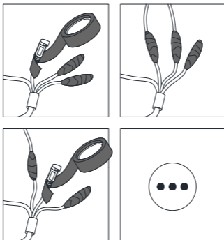
Figure 2-27 Waterproof Cables
