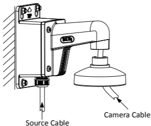
Figure 2-16 Cable Routing
